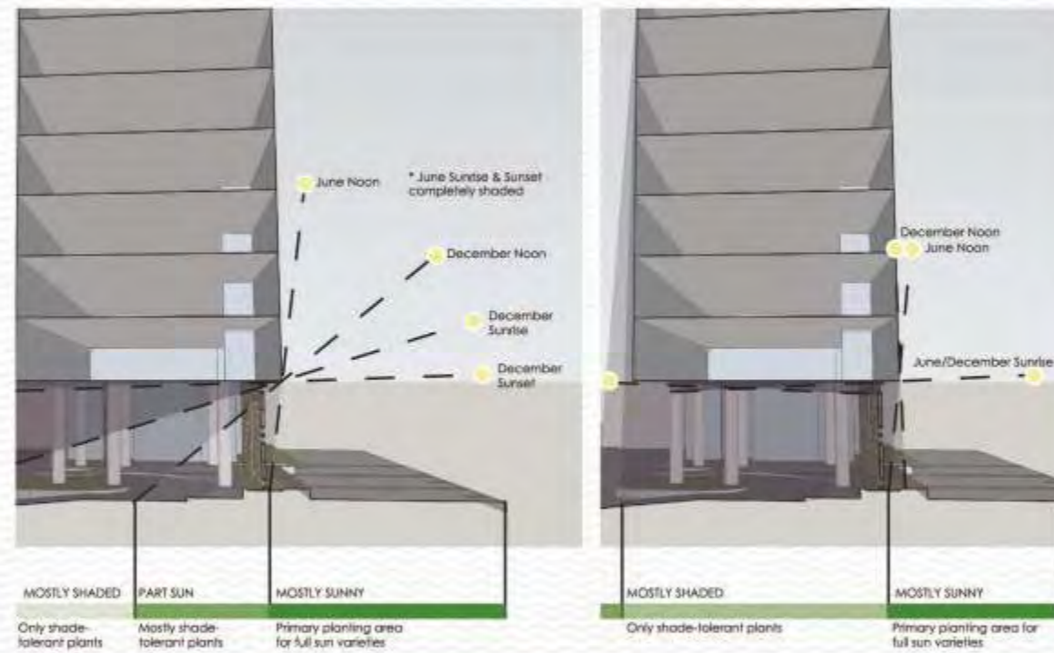
Typical entry sun shade study
